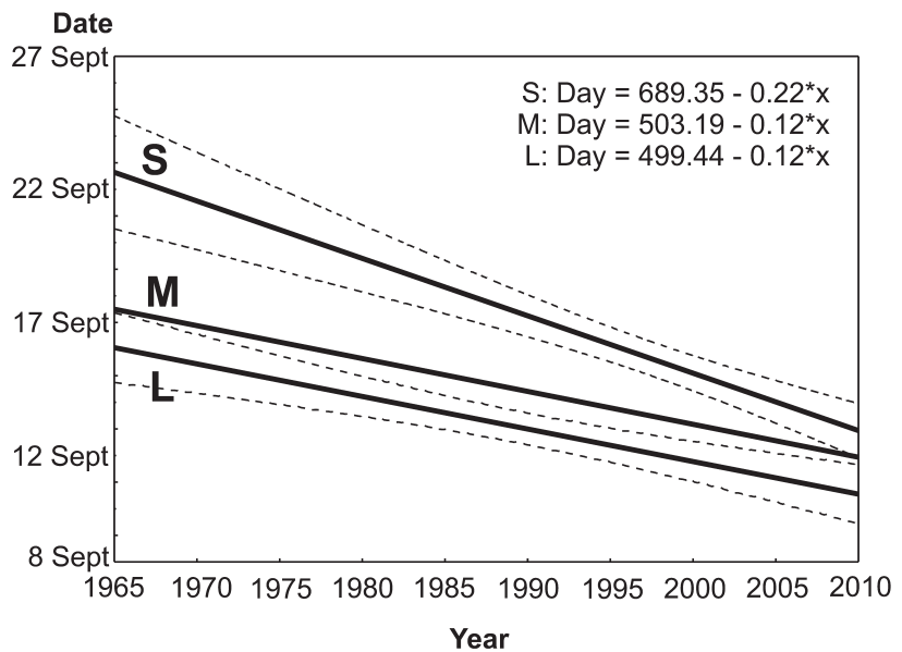
Fig. 2. Temporal trends in autumn migration timing of short-, medium and long-winged Blackcaps captured during autumn migration on the Polish Baltic coast during 1967–2006 (S, M, L – short-, medium- and long-winged Blackcaps, respectively; bold line – regression lines for short-, medium- and long-winged individuals; dashed lines – 95% confidence interval, not-shown for clarity in medium-winged birds).
