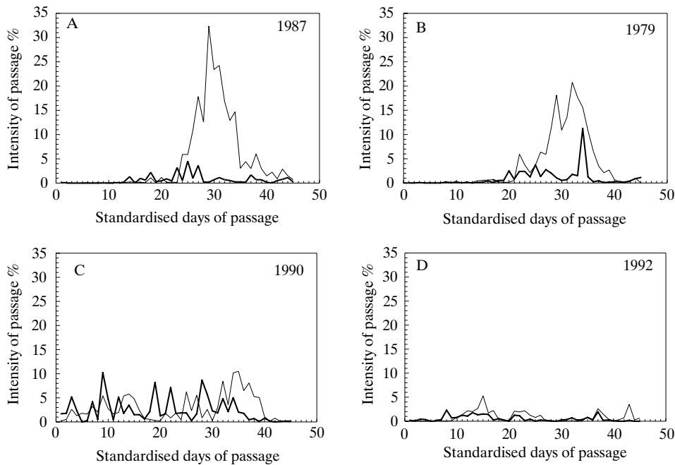
Fig. 3. Comparison of migration dynamics at the Mierzeja Wiślana station – thick line – and in the region (mean result for remaining stations) – thin line; subsequent figures present years with: A – migration that is very intensive in the region but very weak at MW, B – migration that is intensive in the region and weak at MW, C – intensive migration at all stations, D – very weak migration at all stations. The first standardised day of passage at MW = 17 Sep.; migration intensity measured as percentage of birds caught on a given day in relation to the mean number of birds in autumn seasons 1979-1993.
