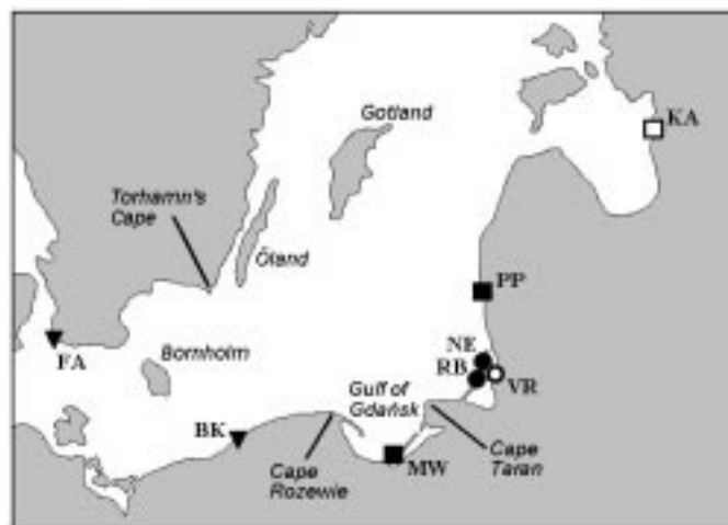
Fig. 1. Location of the bird ringing stations from which the material used in the paper originates: KA – Kabli (58°01'N, 24°27'E), PP – Pape (56°11'N, 21°03'E), NE – Neringa (55°27'N, 21°04'E), VR – Ventes Ragas (55°21'N, 21°12'E), RB – Rybachy (55°09'N, 20°52'E), MW – Mierzeja Wiślana (54°21'N, 19°19'E), BK – Bukowo-Kopań (54°28'N, 16°25'E), FA – Falsterbo (55°22'N, 12°52'E). Squares – stations from which data were used only in comparisons of migration dynamics; circles – stations from which data were used in comparisons of migration dynamics and ringing recoveries; open signs – data were used only in comparisons of multi-year migration dynamics; black signs – data were used in comparisons of multi-year and seasonal migration dynamics; triangles – remaining stations.
