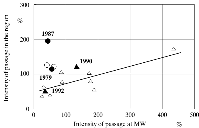
Fig. 2. Correlation of migration intensity (measured by number of birds caught in given year in relation to multi-year mean) at Mierzeja Wiślana and in the region (mean result at remaining stations – KA + PP + NE + VR + RB). Circles – outstanding years; black signs – years for which the seasonal dynamics are presented in Figure 3; the trend line drawn excludes the outstanding years; for station symbols see Fig. 1.
